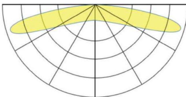
Beam Angle: 175°
